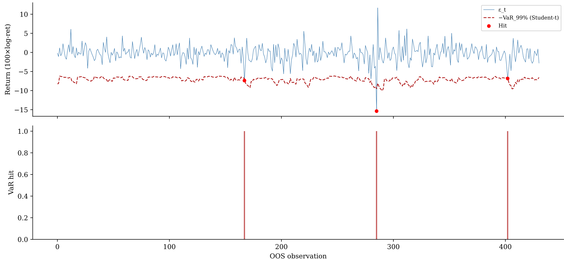
LSTM-SSE-t-Student — BTC-USD VaR 99% Hit Sequence
